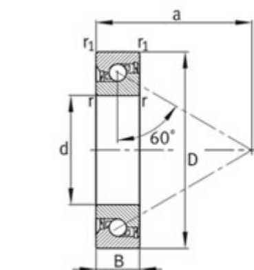
7602..-2RS, 7603..-2RS, BSB..-2RS
